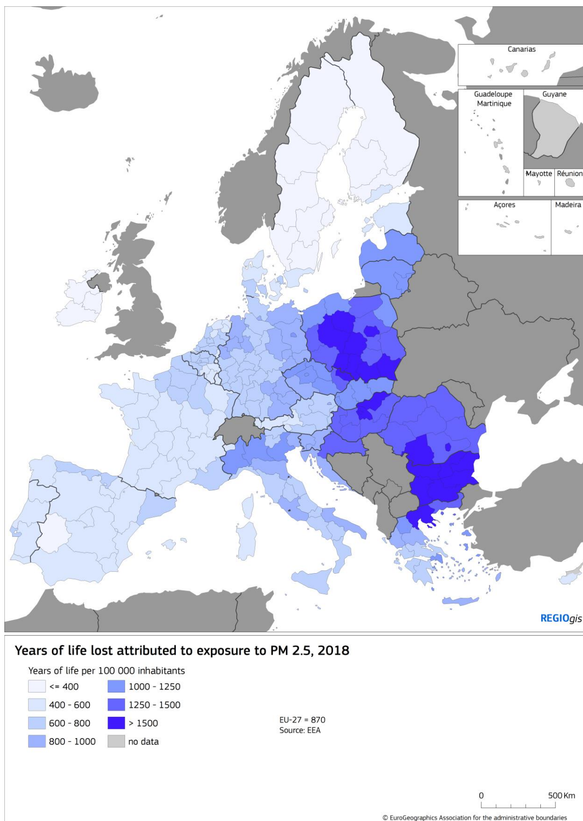
Map 3-12 Years of life lost due to exposure to PM2.5, 2018
