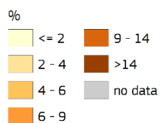
Artificial areas with ecosystem deficit, 2012
