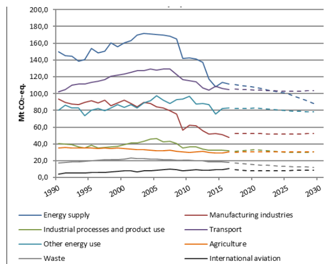
Figure 10: Greenhouse gas emissions by sector (Mt. CO 2 -eq.). Historical data 1990-2015. Projections 2016-2030 63
