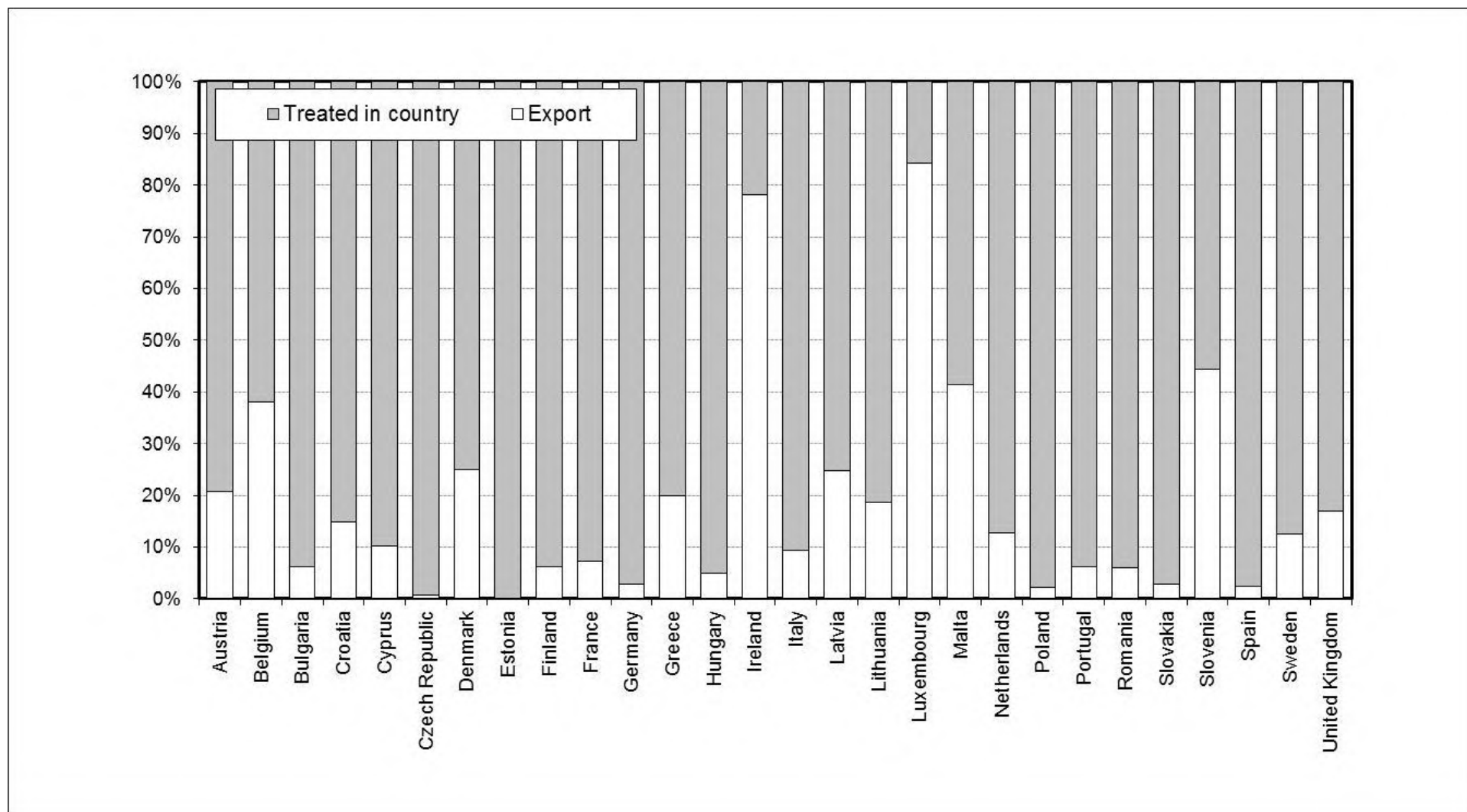
Figure 2.4: Export of Hazardous Waste out of Each Member State in Relation to Generation in 2015, in % distribution
