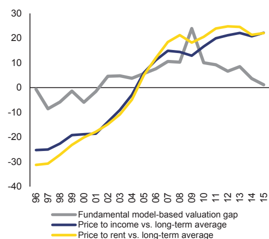
Graph 1.11: Valuation gaps: price/income, price/rent and fundamental model
