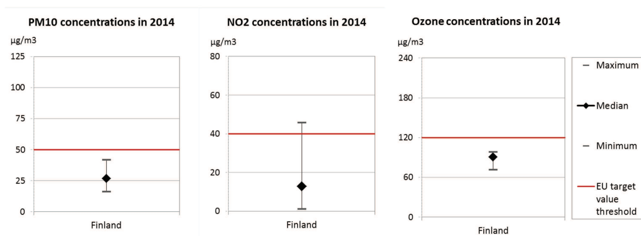
Figure 9: Attainment situation for PM10, NO2 and O3 in 2014 in Finland
