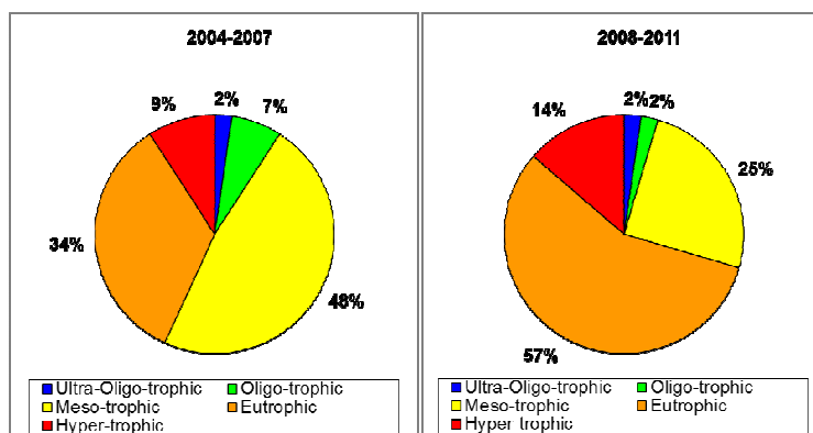
Figure 5. Coastal water eutrophication classification during the 2004-2007 and 2008-2011 reporting periods.
