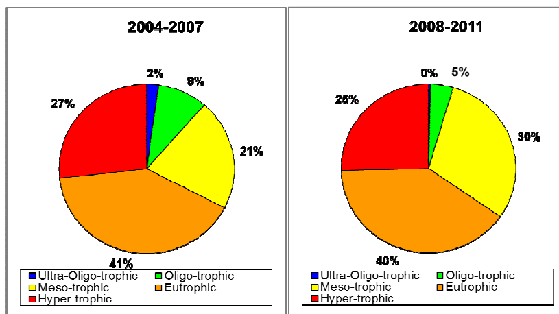
Figure 5. Surface fresh waters eutrophication classification during the 2004-2007 and 2008-2011 reporting periods.
