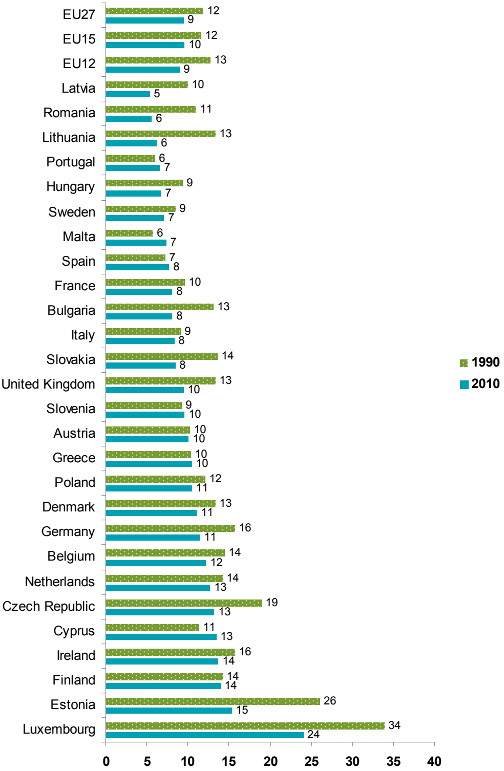
Figure 2: Greenhouse gas emissions (tCO 2 -eq.) per capita of Member States for 1990 and 2010
