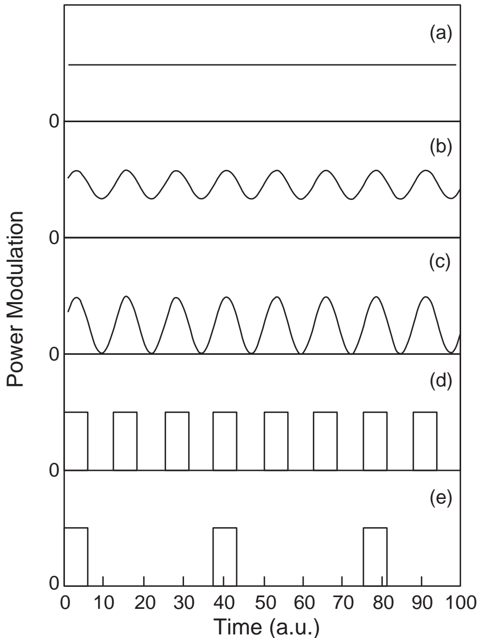
Figure 1.1. Some types of power modulation used in biological experiments. (a) Continuous wave; (b) sinusoidal modulation with a modulation index < 1 ; (c) sinusoidal modulation with a modulation index of 1; (d) 100% square-wave modulated wave; (e) pulse modulated wave, where duty cycle and pulse width are different. Time is expressed in arbitrary units (a.u.).
