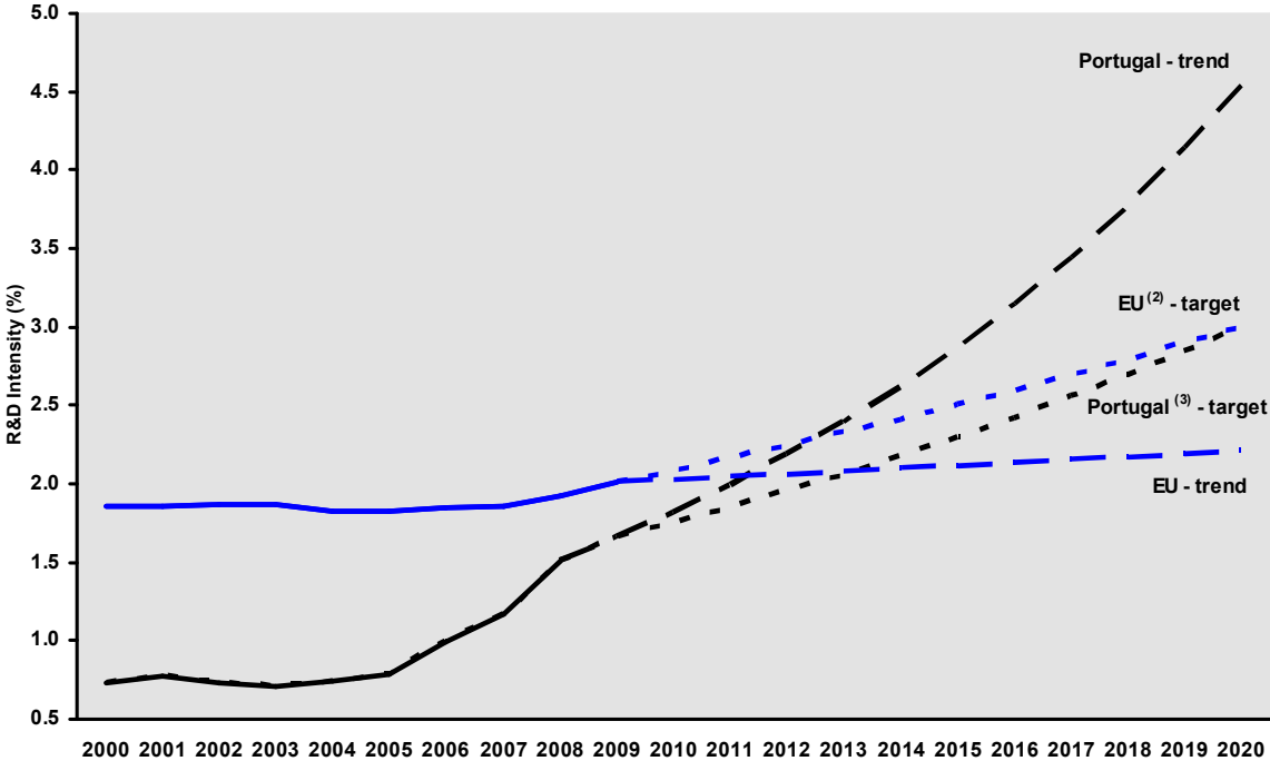
Portugal - R&D Intensity projections, 2000-2020 (1)
