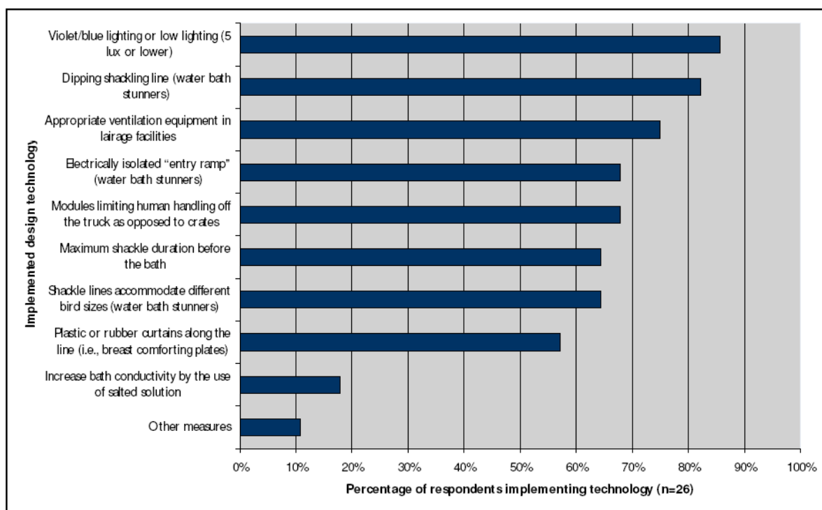
Figure 2 – Additional technologies implemented by the poultry industry for waterbath
