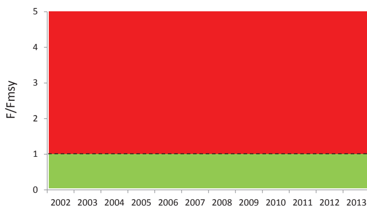
Figure A8.17 Trend in total landings (top graph), SSB (middle graph) and evolution of the ratio F/F_{MSY} over time (bottom graph; red area means overfishing as F > F_{MSY} and green area means sustainable as F < F_{MSY} ) for Red mullet in GSA 6 (Northern Spain).
