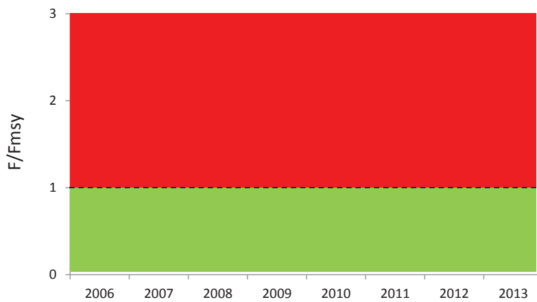
Figure A8.15 Trend in total landings (top graph), SSB (middle graph) and evolution of the ratio F/F_{MSY} over time (bottom graph; red area means overfishing as current F > F_{MSY} and green area means sustainable as F < F_{MSY} ) for Norway lobster in GSA 9 (Ligurian and North Tyrrhenian Seas).
