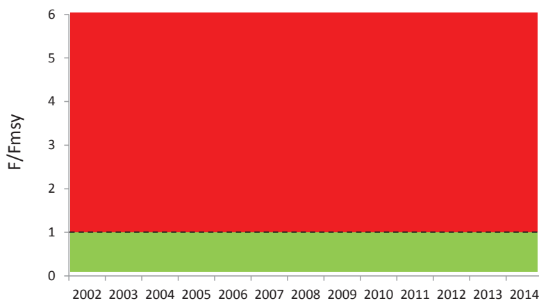
Figure A8.4 Trend in total landings (top graph), SSB (middle graph) and evolution of the ratio F/F_{MSY} over time (bottom graph; red area means overfishing as current F > F_{MSY} and green area means sustainable as F < F_{MSY} ) for Blue and red shrimp in GSA 6 (Northern Spain).
