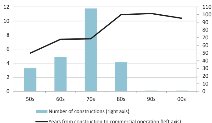
Figure 10 Duration of NPPs construction in Europe 43
