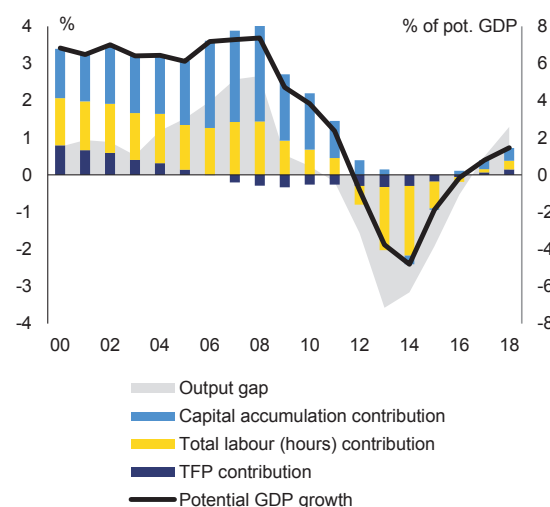
Graph 1.5: Potential output
