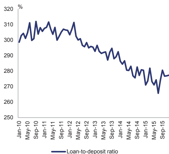
Graph 2.3.9: Funding developments
