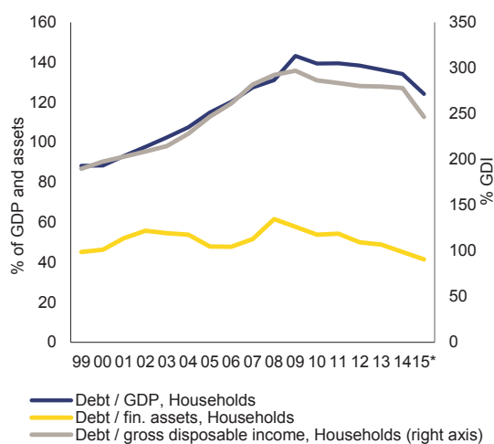
Graph 2.3.6: Leverage, Households
