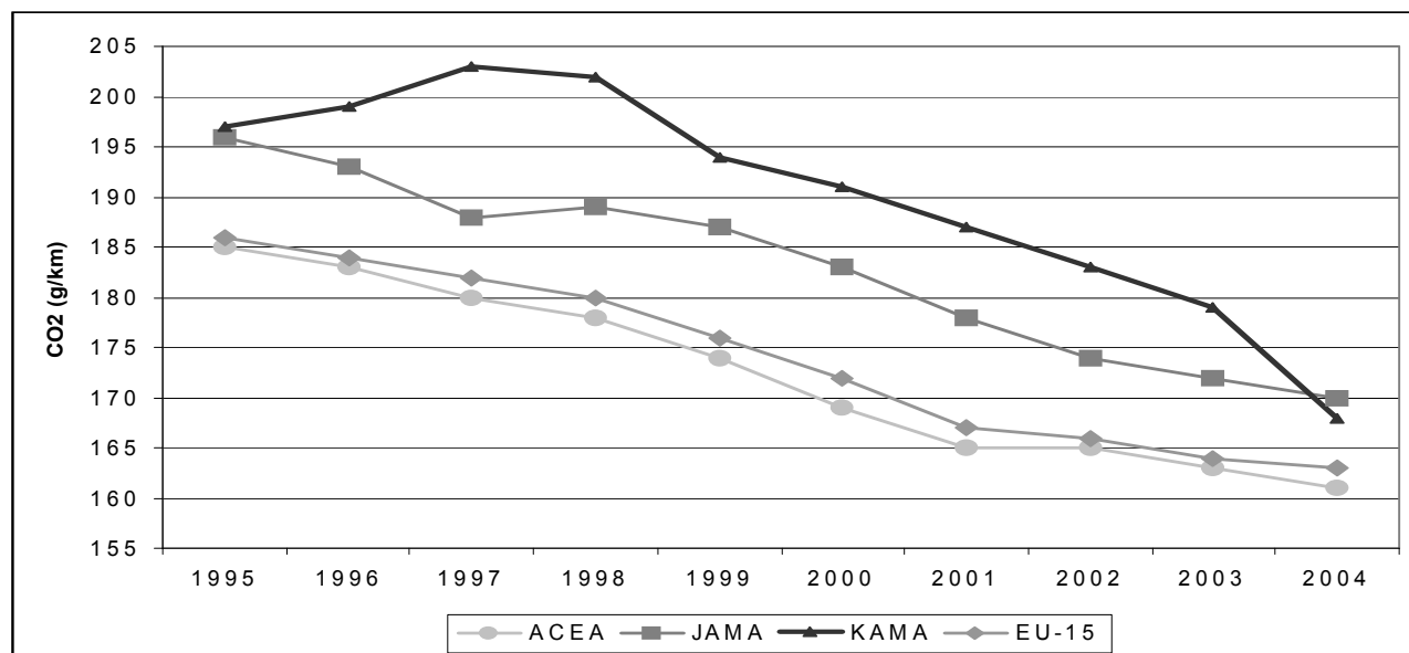
Figure 8: Evolution of CO 2 emissions from new passenger cars
