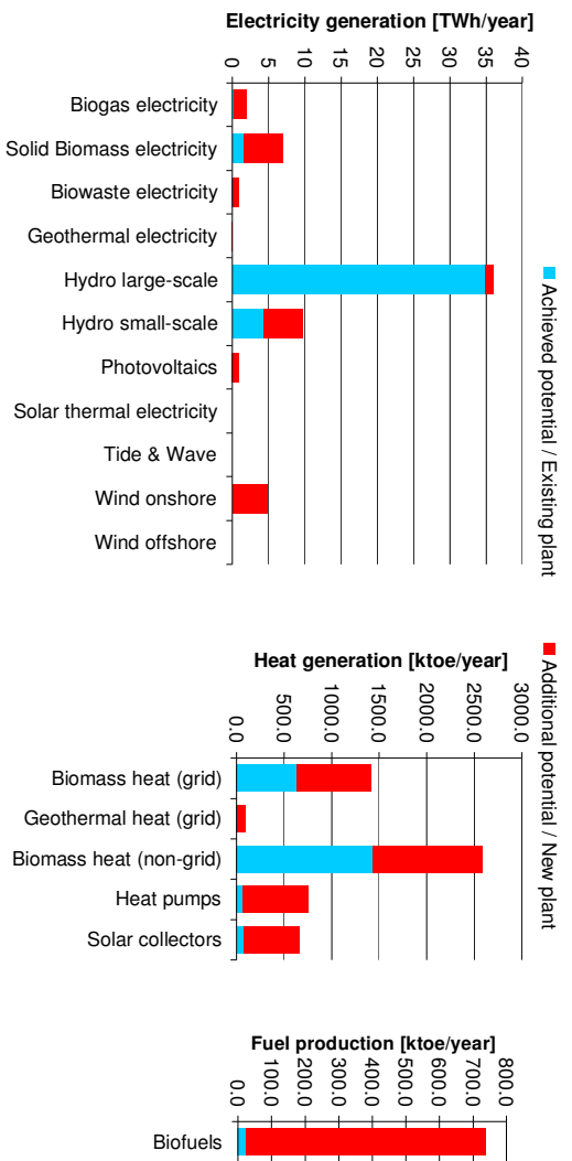
Figure 3: Mid-term potentials of RES electricity, heat and transport in Austria
