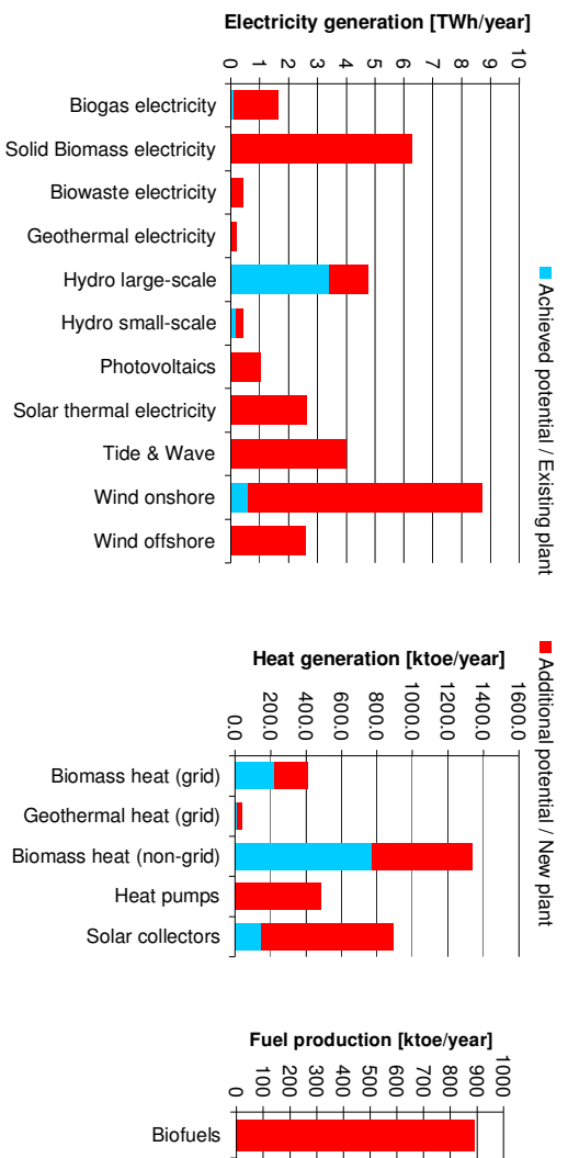
Figure 3: Mid-term potentials of RES electricity, heat and transport in Greece
