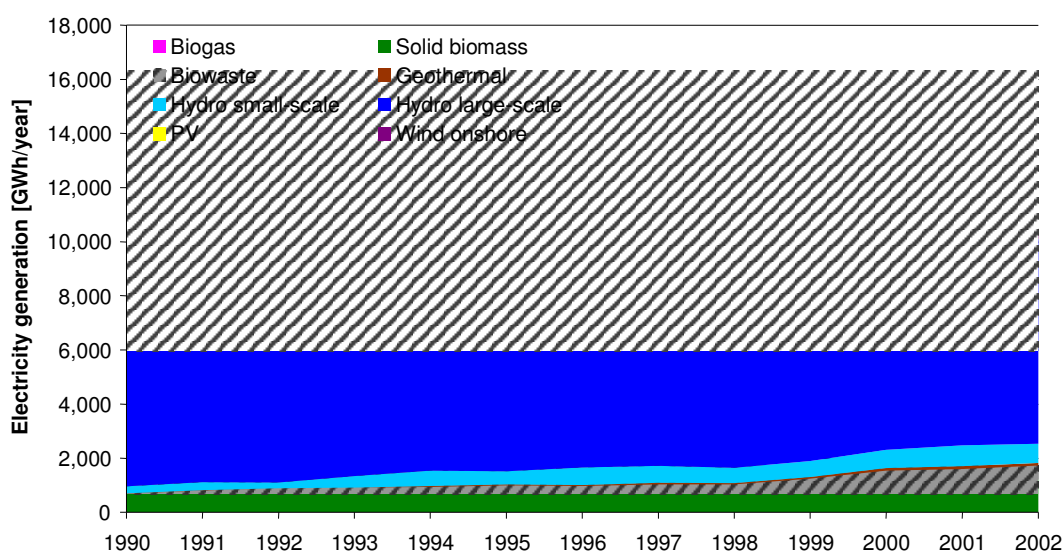
Figure 1: RES-electricity production up until 2002 26 in Portugal
