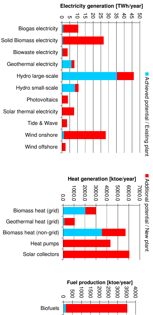
Figure 3: Mid-term potentials of RES electricity heat and transport in Italy
