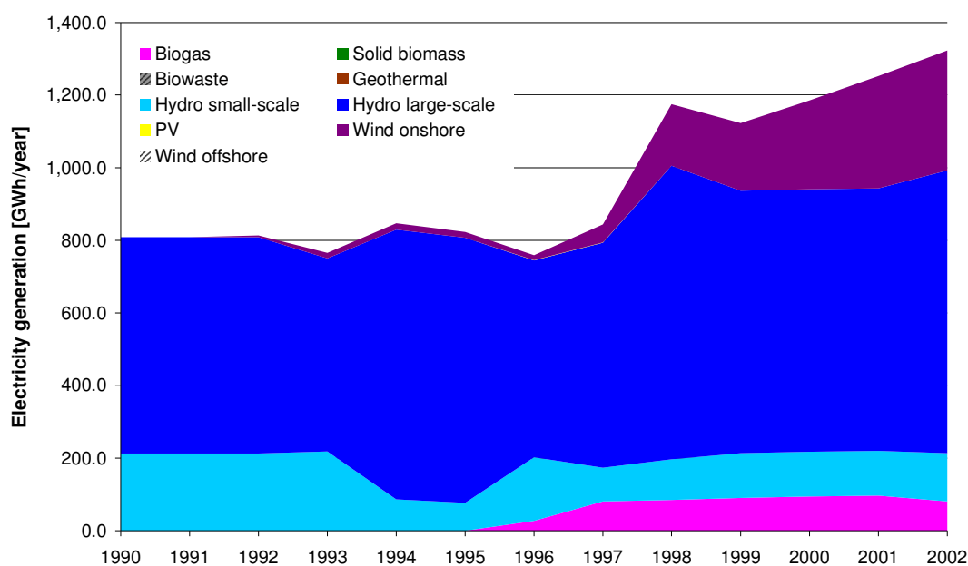
Figure 1: RES-electricity production up until 2002 18
