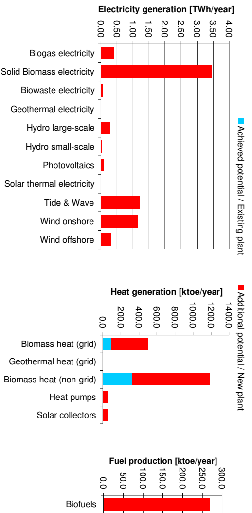
Figure 2: Mid-term potentials of RES electricity, heat and transport in Estonia
