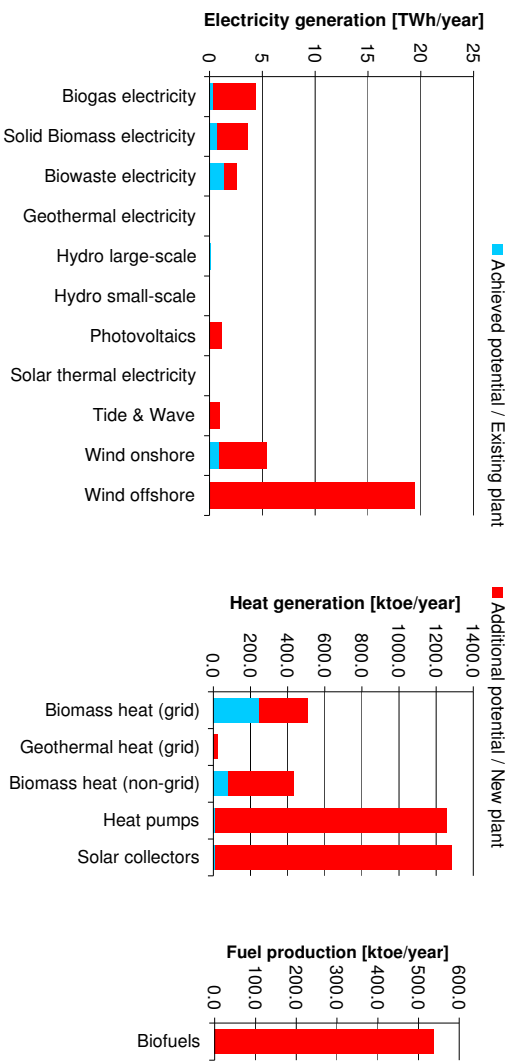
Figure 2: Mid-term potentials of RES electricity heat and transport in the Netherlands
