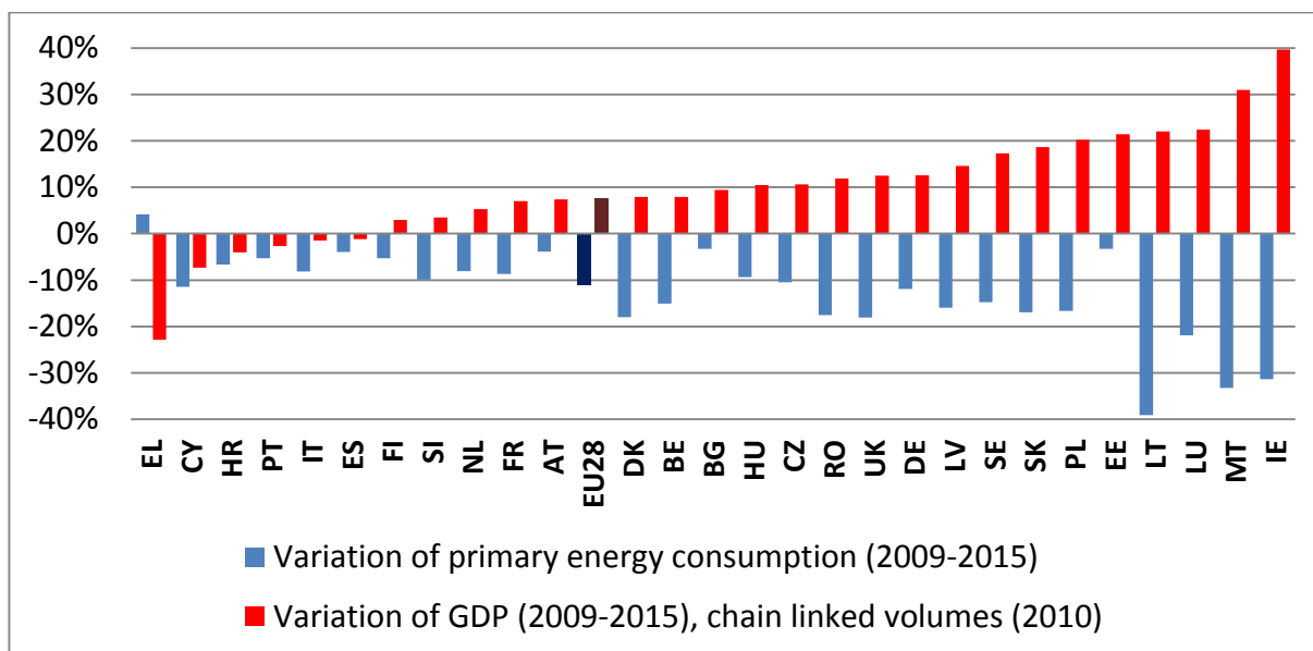
Figure 2: GDP and primary energy consumption, 2009-2015
