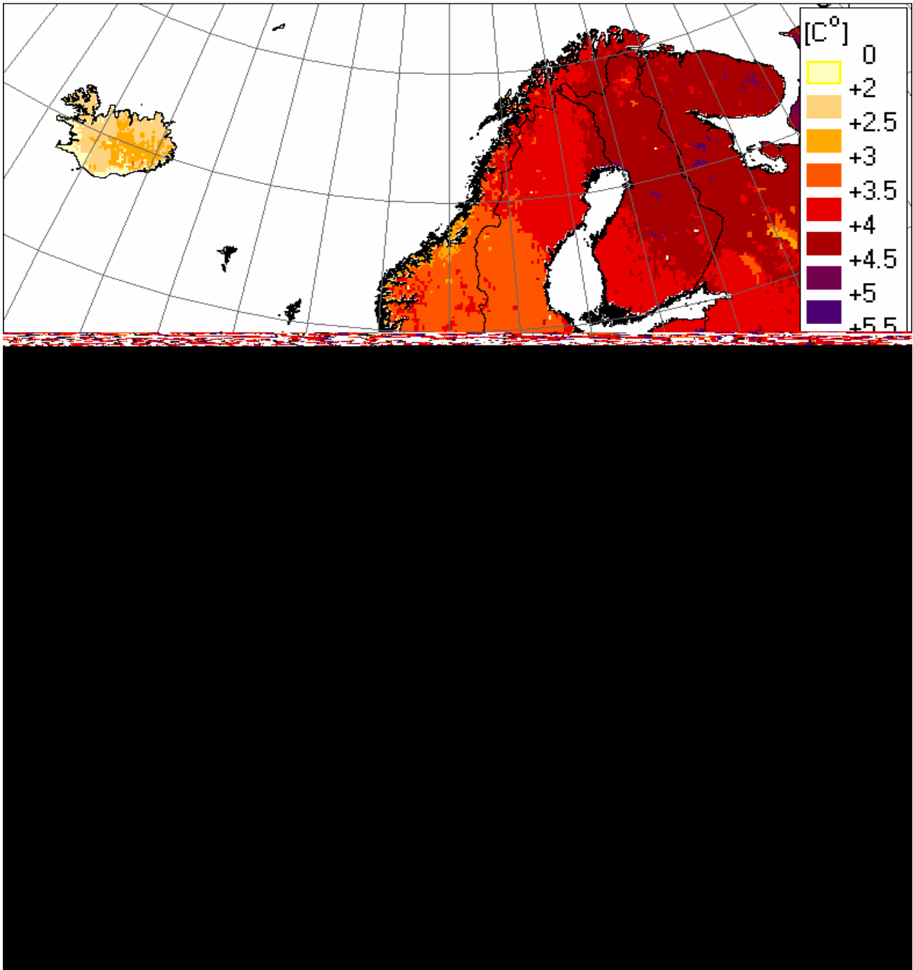
Temperature: change in mean annual temperature [C°]
